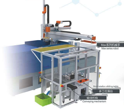
护目镜防护膜IMD 智能产线系统 IMD intelligent production line system of protective film for goggles
