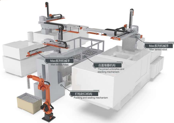
1出16 培养皿智能产线系统 Petri dish intelligent production line system of 16 cavities
